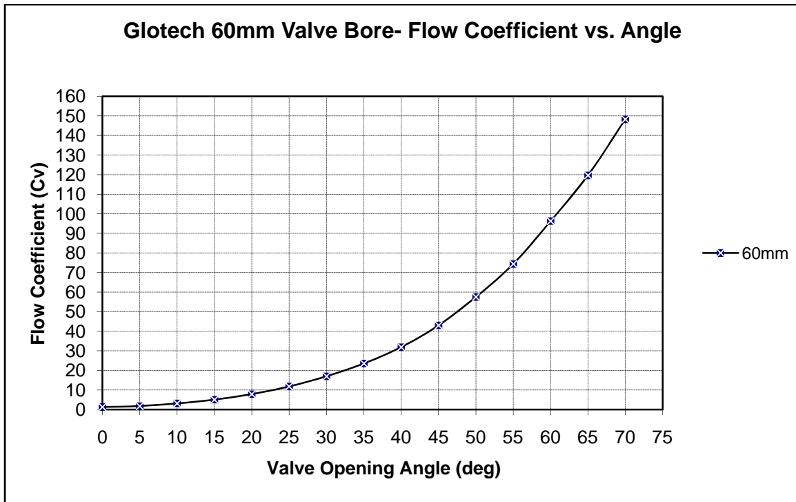
Figure 1-1. Flow Coefficient vs. Valve Opening Angle
