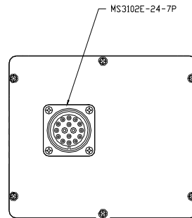
Figure 2-1. Glo-Tech 60 mm Bypass Valve Outline Drawing
